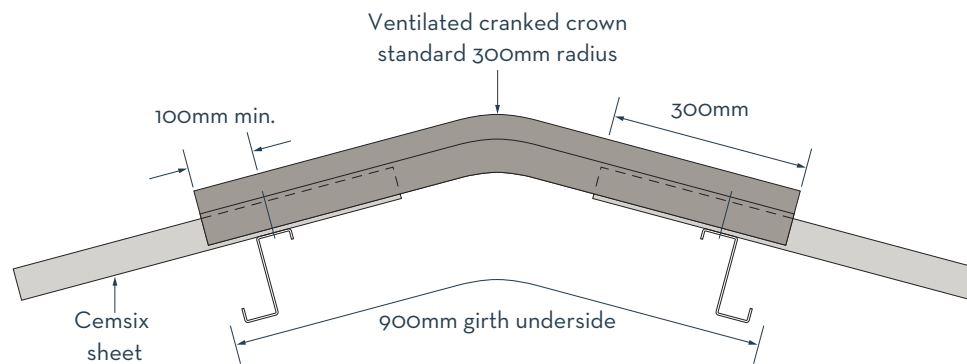
Cranked crown ventilation ridge
