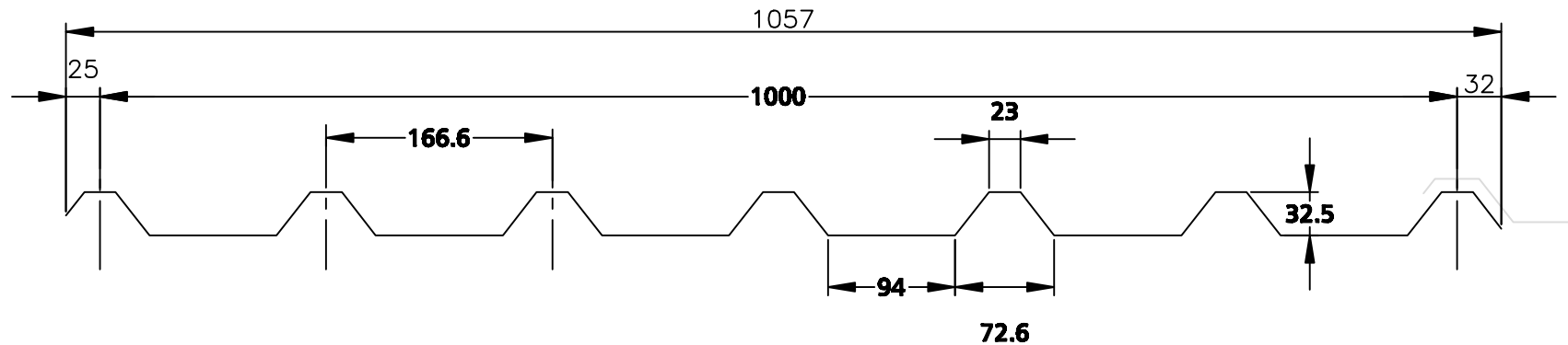
EUROCLAD 32/1000 FORWARD SPECIAL - ROOF PROFILE FILON CODE: 283C OVERALL WIDTH: 1057
